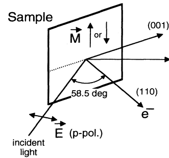
FIG. 2. Experimental geometry used in spin-polarized photoemission measurements.
