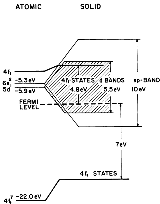
FIG. 11. Simplified model for Gd used to estimate the weights of the various transitions that contribute to \langle \sigma_{xy}^{(2)} \rangle .
