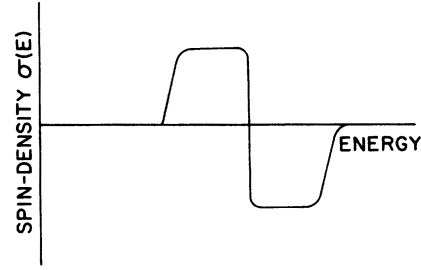
FIG. 15. Schematic representation of the net spin density expected from the Stoner model as a function of energy for a particular band when an exchange splitting exists.
