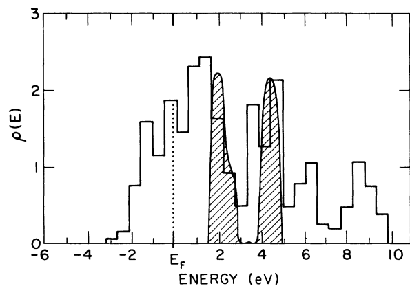
FIG. 10. Density of states of Gd metal. Histogram is as calculated by Dimmock et al. (Ref. 1) and hatched curve is the approximate density of states as determined experimentally by the magneto-optic Kerr effect. Experimental result covers only the range shown.
