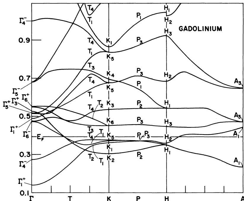
FIG. 9. Band structure of Gd metal [Dimmock et al. (Ref. 1)]. Note the flatness of the d bands.
