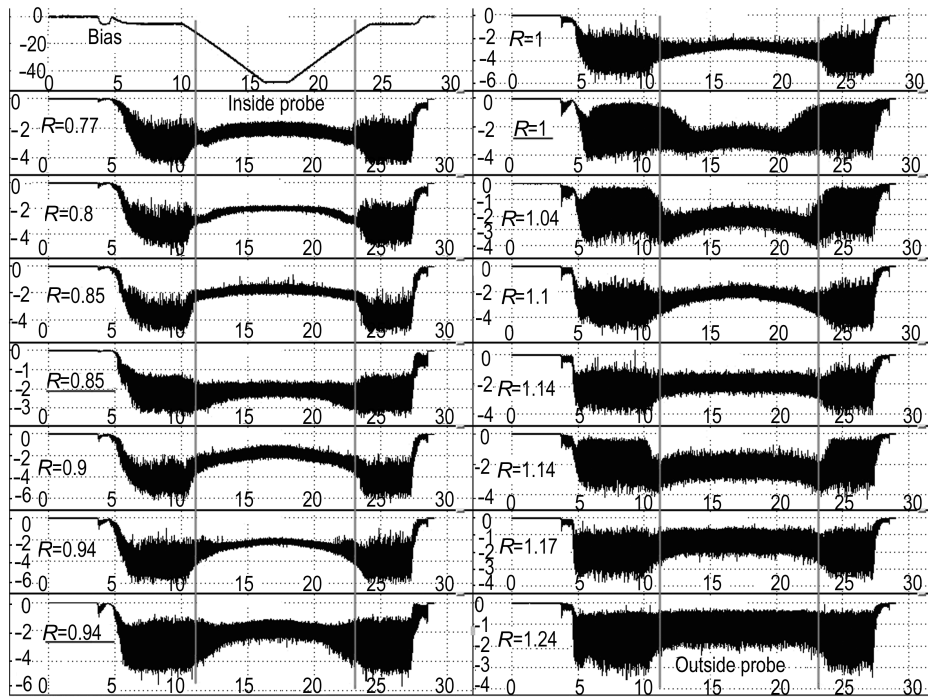
Fig. 2 Ion saturation current (a.u.) to a selection of probes across the radius as the bias on plates 2 is swept to -50 V (top left panel), time from 0 s to 30 s. Underlined radii from probes on bottom plates. The transition (vertical lines) is symmetric, occurring at a voltage near -15 V
