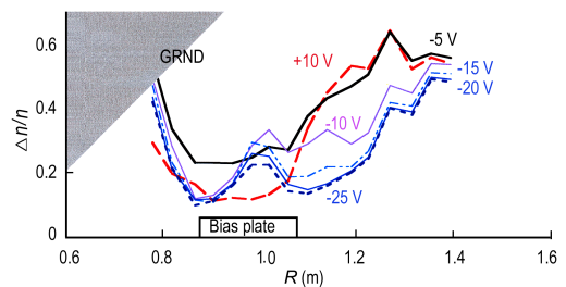
Fig. 4 Profiles of the fractional level of density turbulence (rms) for various applied bias voltages
